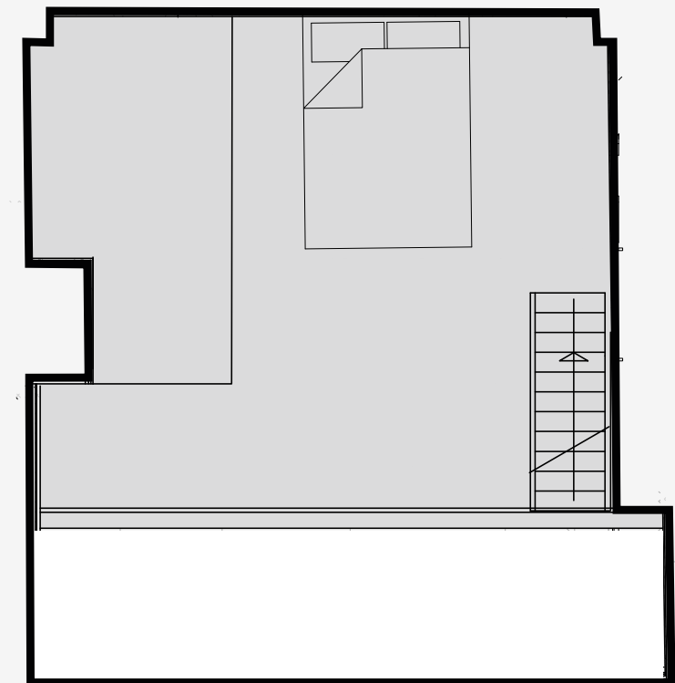
Mezzanine level
